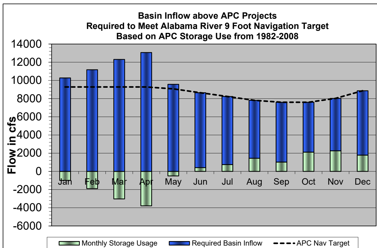
Figure 7-2 Flow Requirements from Rainfall (or Natural Sources) and Reservoir Storage to Achieve the JBT Goal for Navigation Flows for a 9.0-foot Channel
