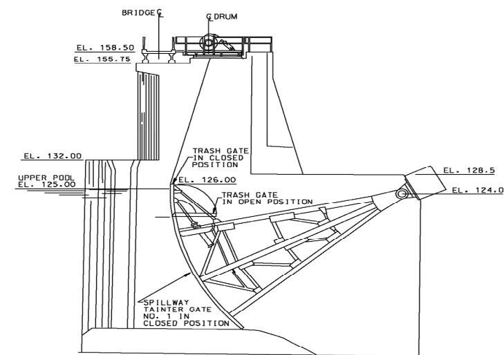
SPILLWAY GATE NO. 1 W/TRASHGATE
