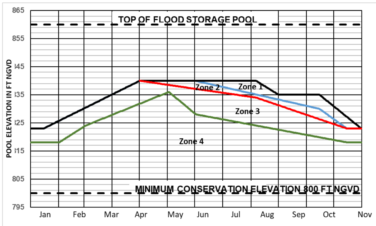
Figure 4. Allatoona Lake Guide Curve and Action Zones
